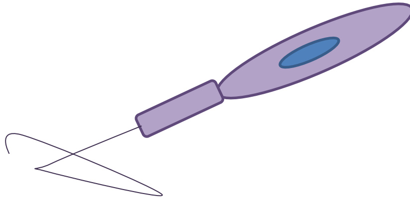
Mature sperm
