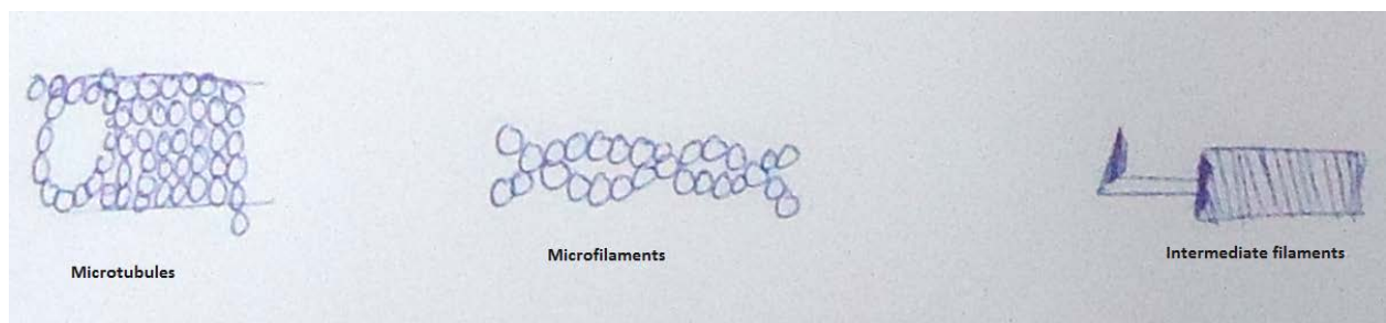
Cytoskeletal fibers
